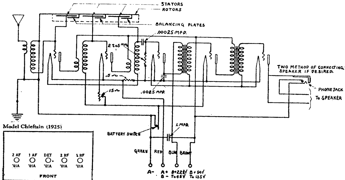
CHIEFTAIN BATTERY OPERATED. -1925-
